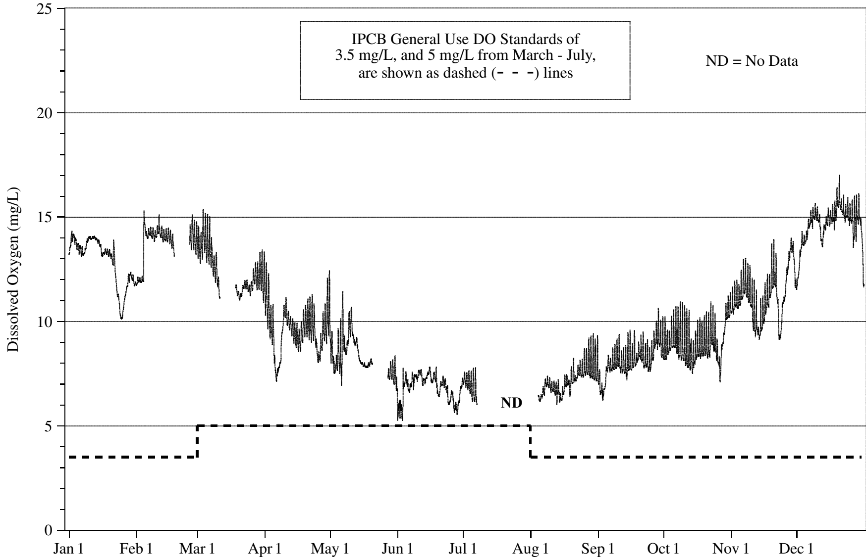
FIGURE 5: DISSOLVED OXYGEN CONCENTRATION MEASURED HOURLY AT OGDEN AVENUE ON THE DES PLAINES RIVER FROM JANUARY 1, 2010, THROUGH DECEMBER 31, 2010
