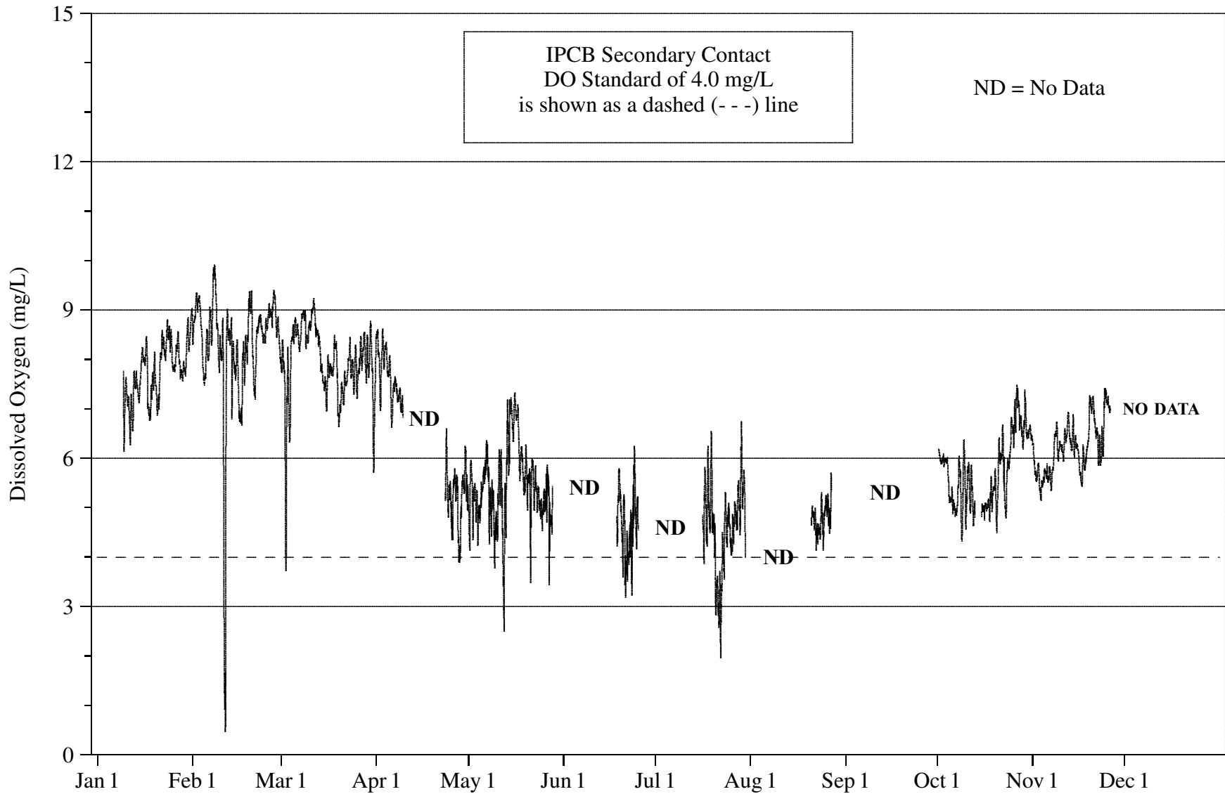
FIGURE 13: DISSOLVED OXYGEN CONCENTRATION MEASURED HOURLY AT ROUTE 83 ON THE CHICAGO SANITARY AND SHIP CANAL FROM JANUARY 1, 2008 THROUGH DECEMBER 31, 2008
