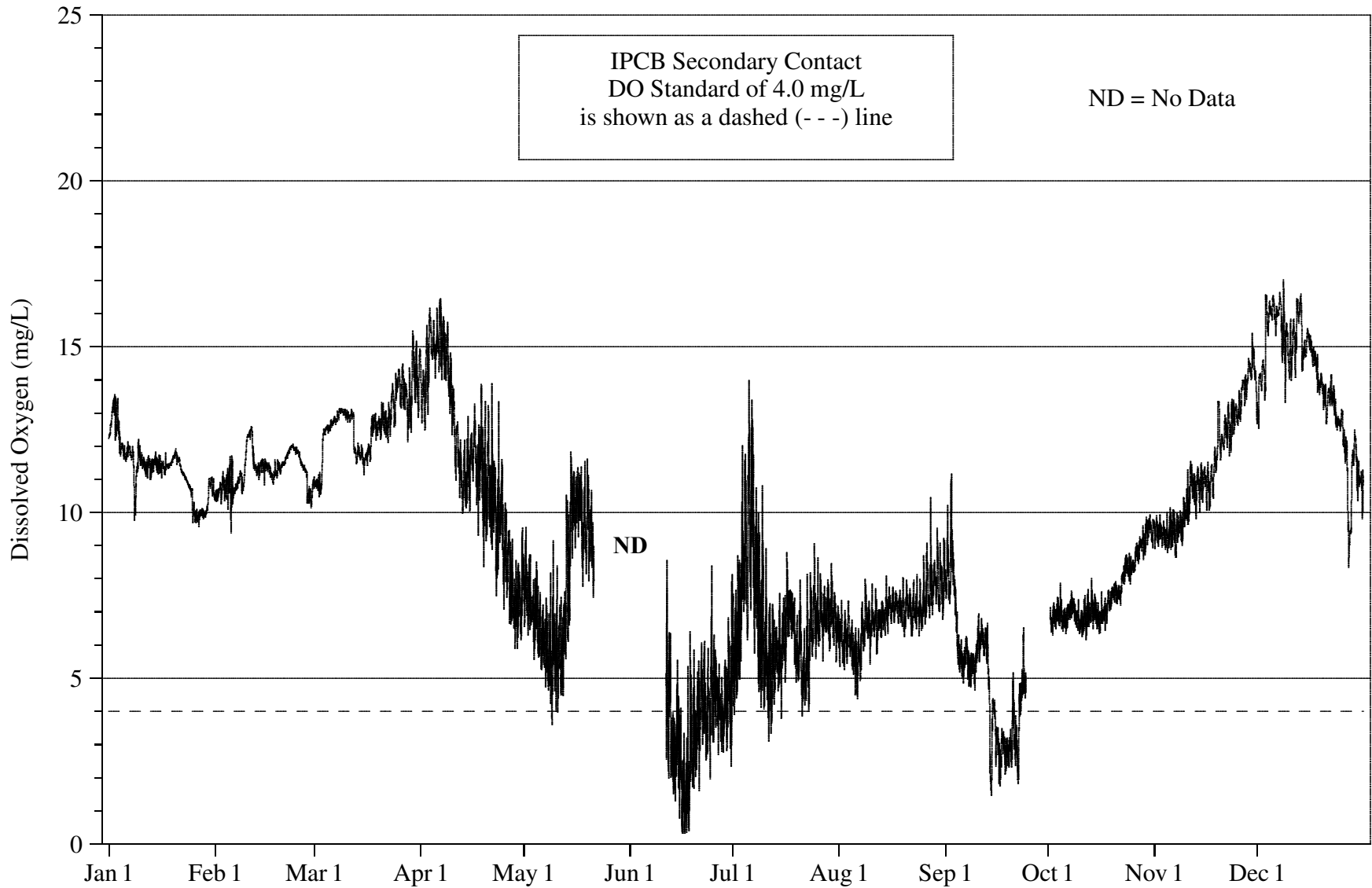
FIGURE 17: DISSOLVED OXYGEN CONCENTRATION MEASURED HOURLY AT C&W INDIANA RAILROAD ON THE LITTLE CALUMET RIVER FROM JANUARY 1, 2008 THROUGH DECEMBER 31, 2008
