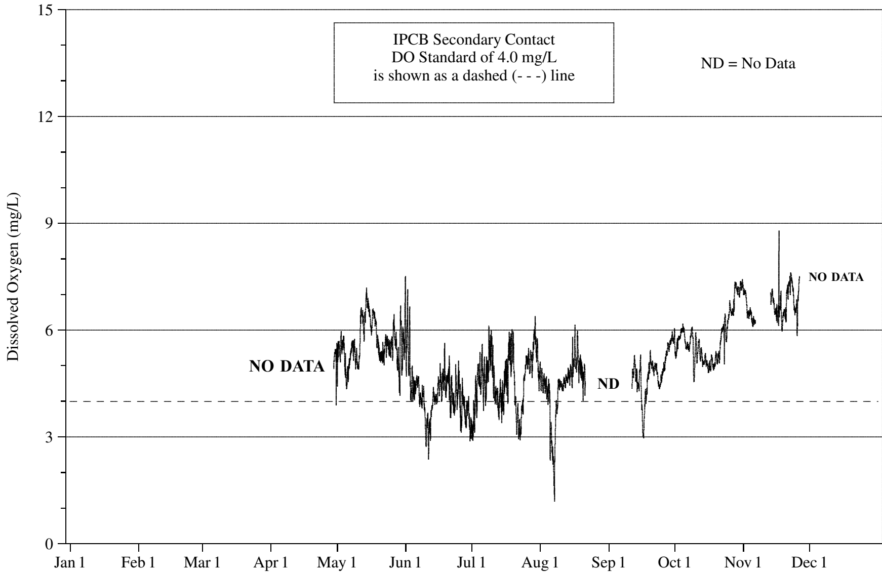
FIGURE 14: DISSOLVED OXYGEN CONCENTRATION MEASURED HOURLY AT ROMEOVILLE ROAD ON THE CHICAGO SANITARY AND SHIP CANAL FROM JANUARY 1, 2008 THROUGH DECEMBER 31, 2008
