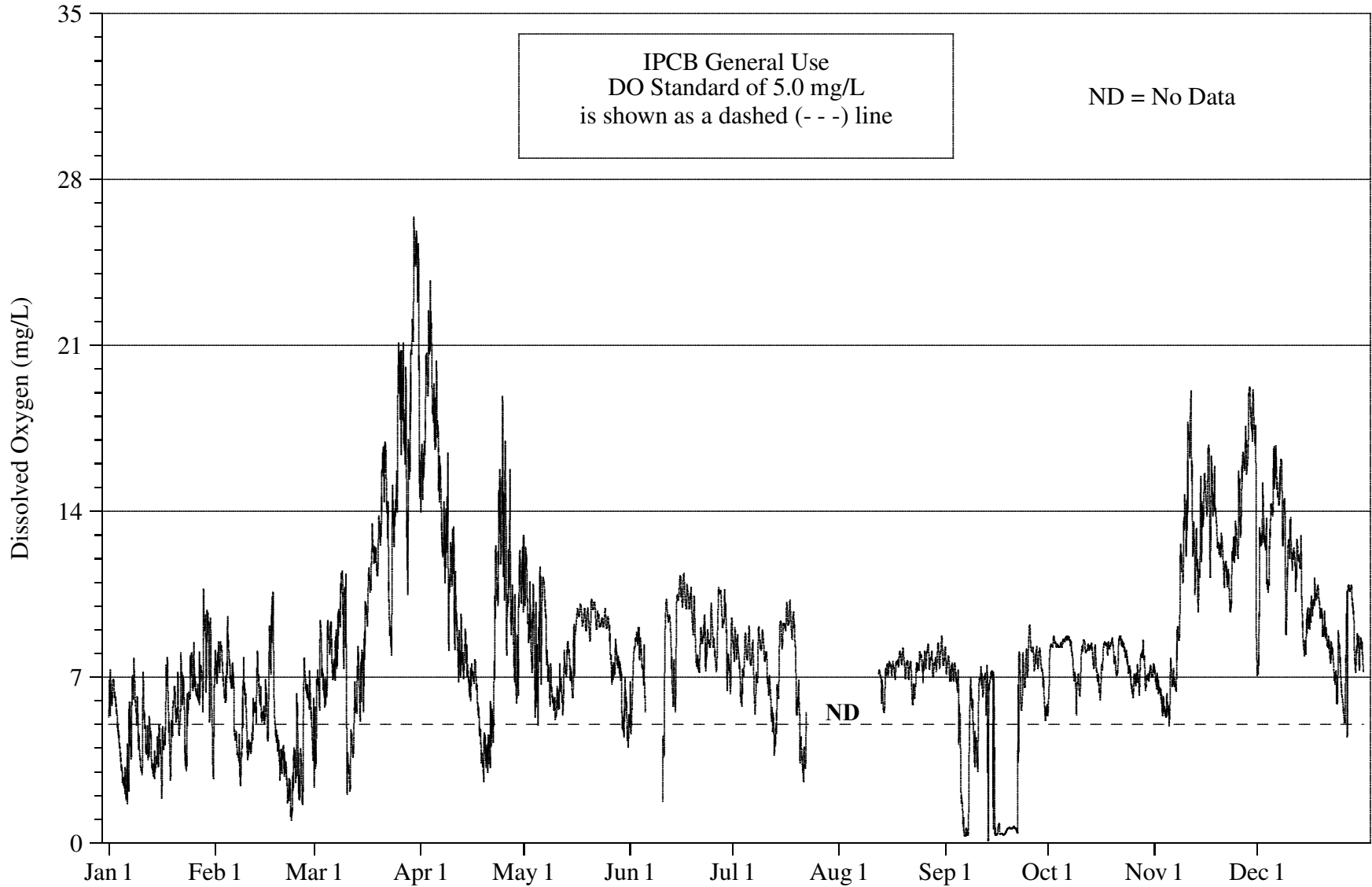
FIGURE 2: DISSOLVED OXYGEN CONCENTRATION MEASURED HOURLY AT MAIN STREET ON THE NORTH SHORE CHANNEL FROM JANUARY 1, 2008 THROUGH DECEMBER 31, 2008
