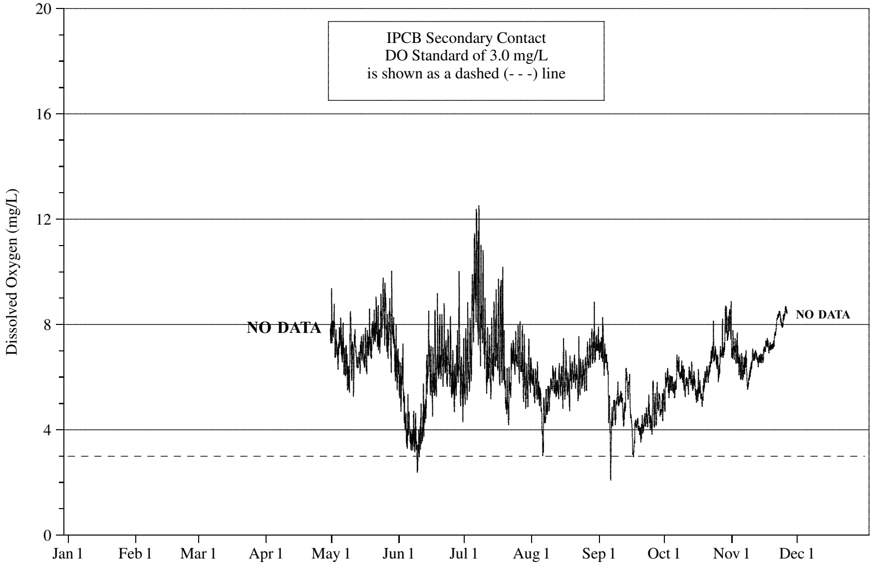
FIGURE 22: DISSOLVED OXYGEN CONCENTRATION MEASURED HOURLY AT SOUTHWEST HIGHWAY ON THE CALUMET-SAG CHANNEL FROM JANUARY 1, 2008 THROUGH DECEMBER 31, 2008
