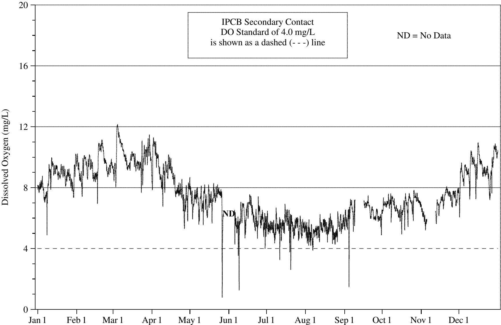
FIGURE 5: DISSOLVED OXYGEN CONCENTRATION MEASURED HOURLY AT FULLERTON AVENUE ON THE NORTH BRANCH CHICAGO RIVER FROM JANUARY 1, 2008 THROUGH DECEMBER 31, 2008
