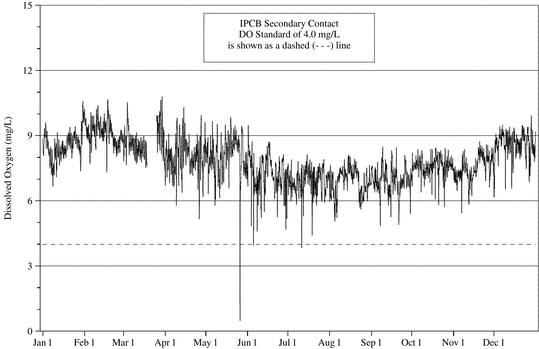
FIGURE 3: DISSOLVED OXYGEN CONCENTRATION MEASURED HOURLY AT FOSTER AVENUE ON THE NORTH SHORE CHANNEL FROM JANUARY 1, 2008 THROUGH DECEMBER 31, 2008
