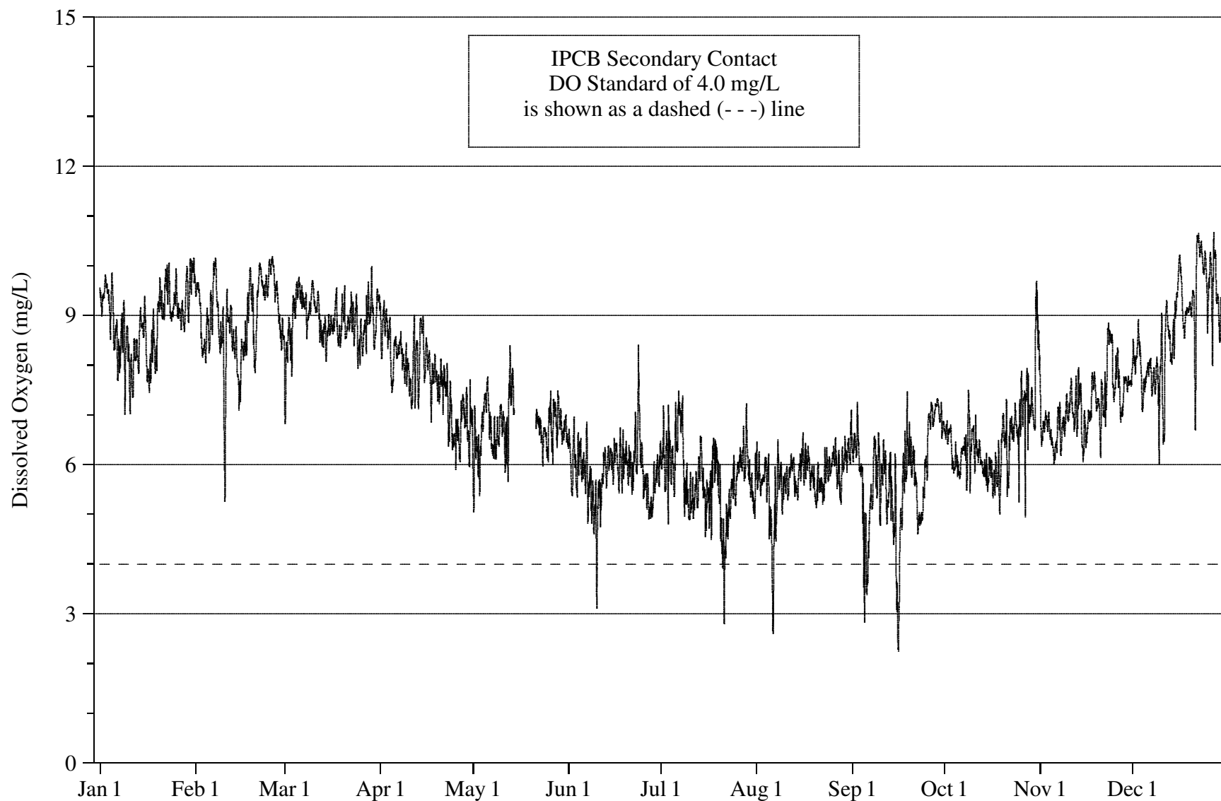
FIGURE 12: DISSOLVED OXYGEN CONCENTRATION MEASURED HOURLY AT B&O CENTRAL RAILROAD ON THE CHICAGO SANITARY AND SHIP CANAL FROM JANUARY 1, 2008 THROUGH DECEMBER 31, 2008
