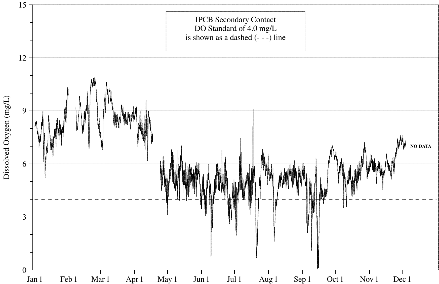
FIGURE 11: DISSOLVED OXYGEN CONCENTRATION MEASURED HOURLY AT CICERO AVENUE ON THE CHICAGO SANITARY AND SHIP CANAL FROM JANUARY 1, 2008 THROUGH DECEMBER 31, 2008
