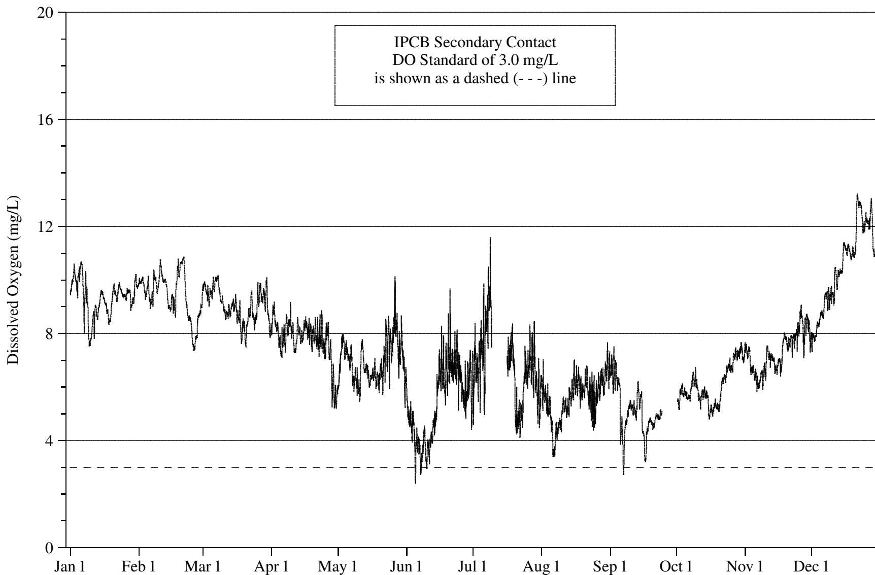
FIGURE 24: DISSOLVED OXYGEN CONCENTRATION MEASURED HOURLY AT ROUTE 83 ON THE CALUMET-SAG CHANNEL FROM JANUARY 1, 2008 THROUGH DECEMBER 31, 2008
