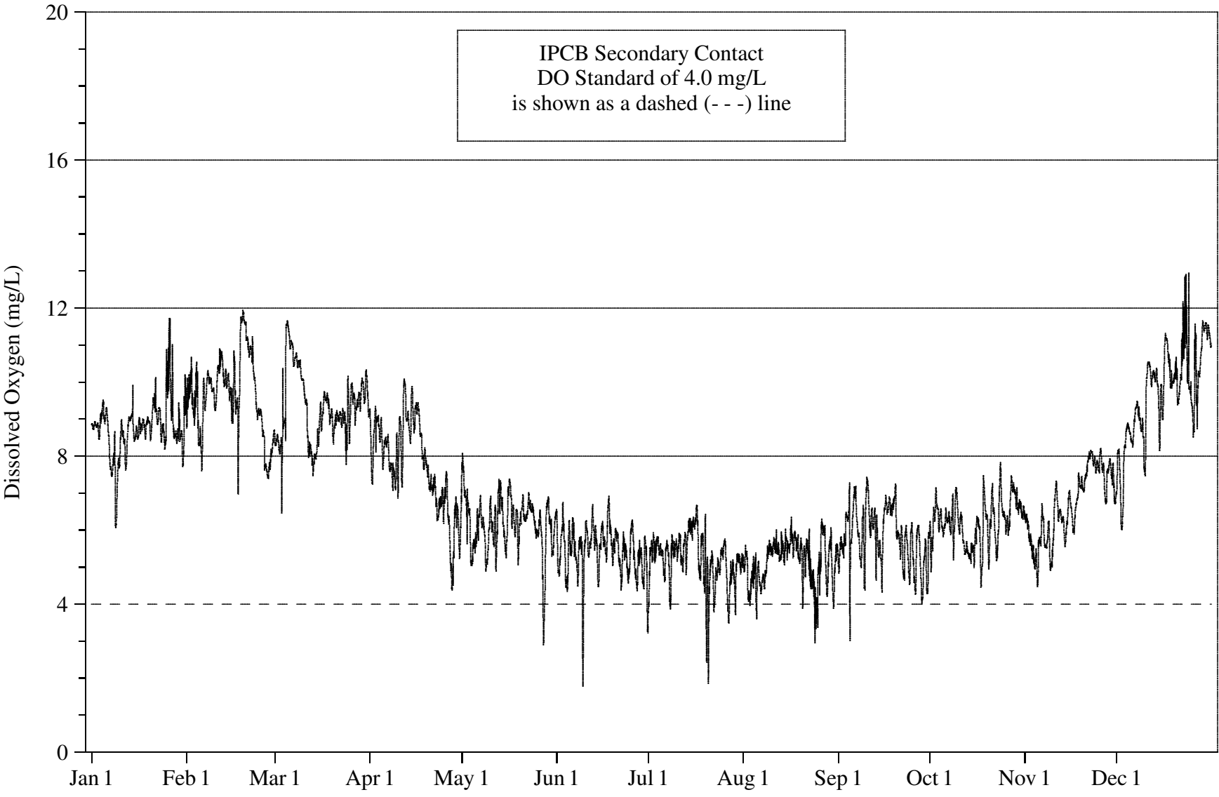
FIGURE 6: DISSOLVED OXYGEN CONCENTRATION MEASURED HOURLY AT KINZIE STREET ON THE NORTH BRANCH CHICAGO RIVER FROM JANUARY 1, 2008 THROUGH DECEMBER 31, 2008
