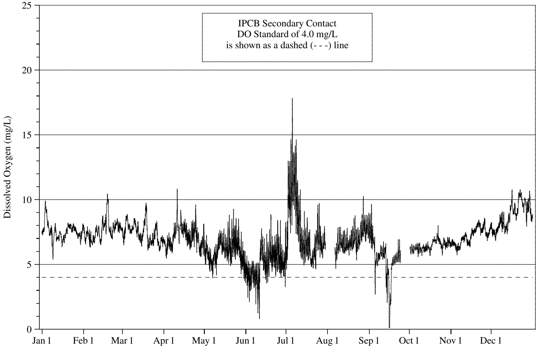
FIGURE 18: DISSOLVED OXYGEN CONCENTRATION MEASURED HOURLY AT HALSTED STREET ON THE LITTLE CALUMET RIVER FROM JANUARY 1, 2008 THROUGH DECEMBER 31, 2008
