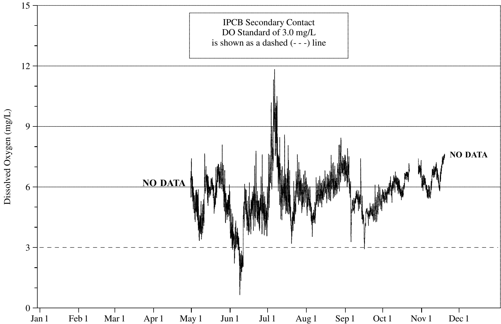
FIGURE 19: DISSOLVED OXYGEN CONCENTRATION MEASURED HOURLY AT DIVISION STREET ON THE CALUMET-SAG CHANNEL FROM JANUARY 1, 2008 THROUGH DECEMBER 31, 2008
