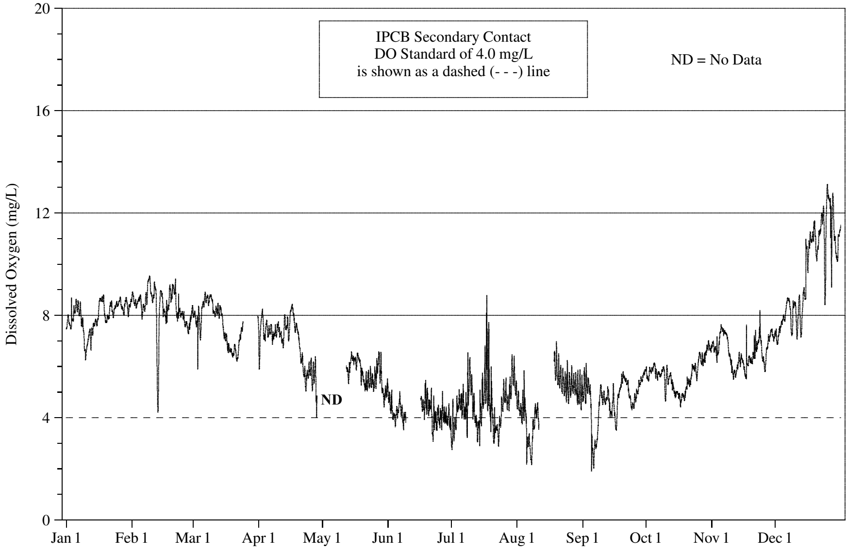
FIGURE 15: DISSOLVED OXYGEN CONCENTRATION MEASURED HOURLY AT LOCKPORT POWERHOUSE ON THE CHICAGO SANITARY AND SHIP CANAL FROM JANUARY 1, 2008 THROUGH DECEMBER 31, 2008
