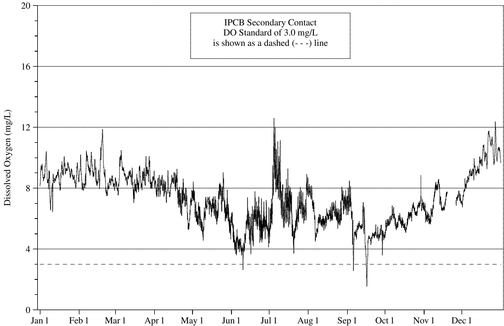
FIGURE 20: DISSOLVED OXYGEN CONCENTRATION MEASURED HOURLY AT CICERO AVENUE ON THE CALUMET-SAG CHANNEL FROM JANUARY 1, 2008 THROUGH DECEMBER 31, 2008
