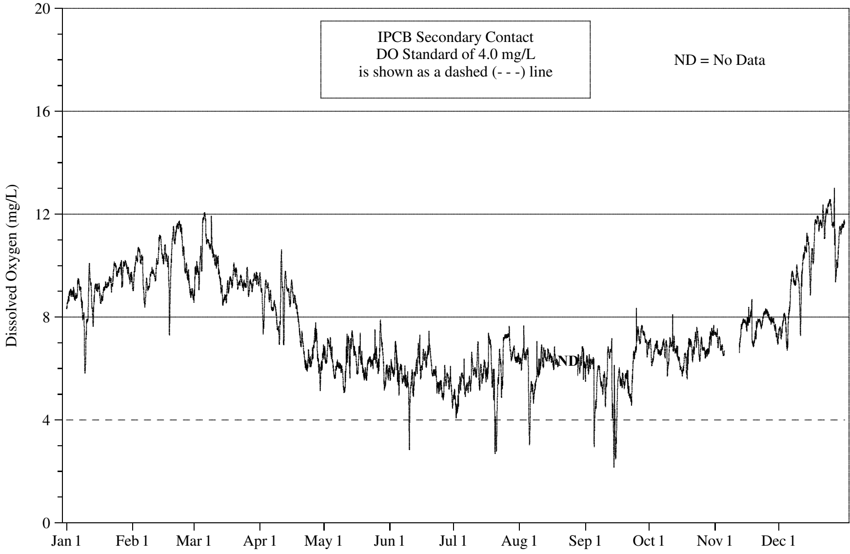
FIGURE 8: DISSOLVED OXYGEN CONCENTRATION MEASURED HOURLY AT LOOMIS STREET ON THE SOUTH BRANCH CHICAGO RIVER FROM JANUARY 1, 2008 THROUGH DECEMBER 31, 2008
