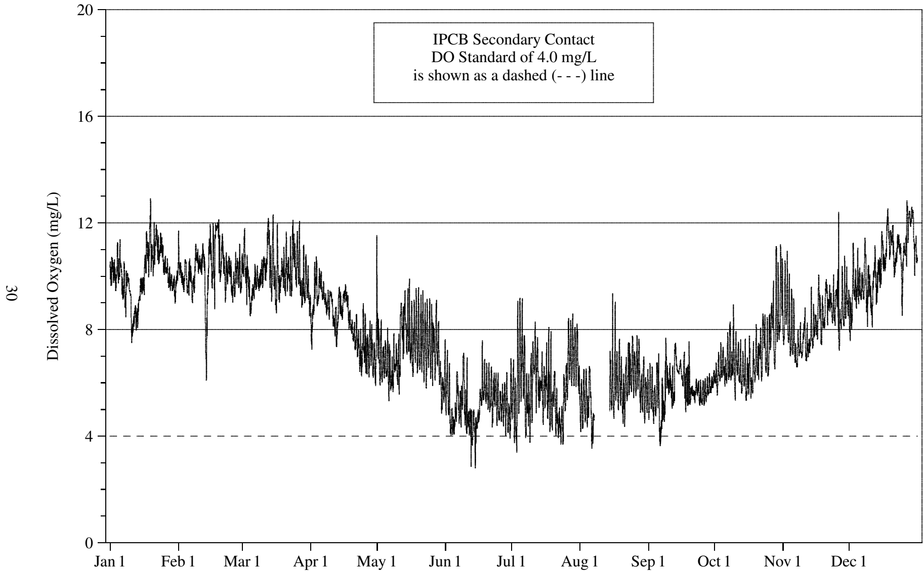
FIGURE 16: DISSOLVED OXYGEN CONCENTRATION MEASURED HOURLY AT JEFFERSON STREET ON THE DES PLAINES RIVER FROM JANUARY 1, 2008 THROUGH DECEMBER 31, 2008
