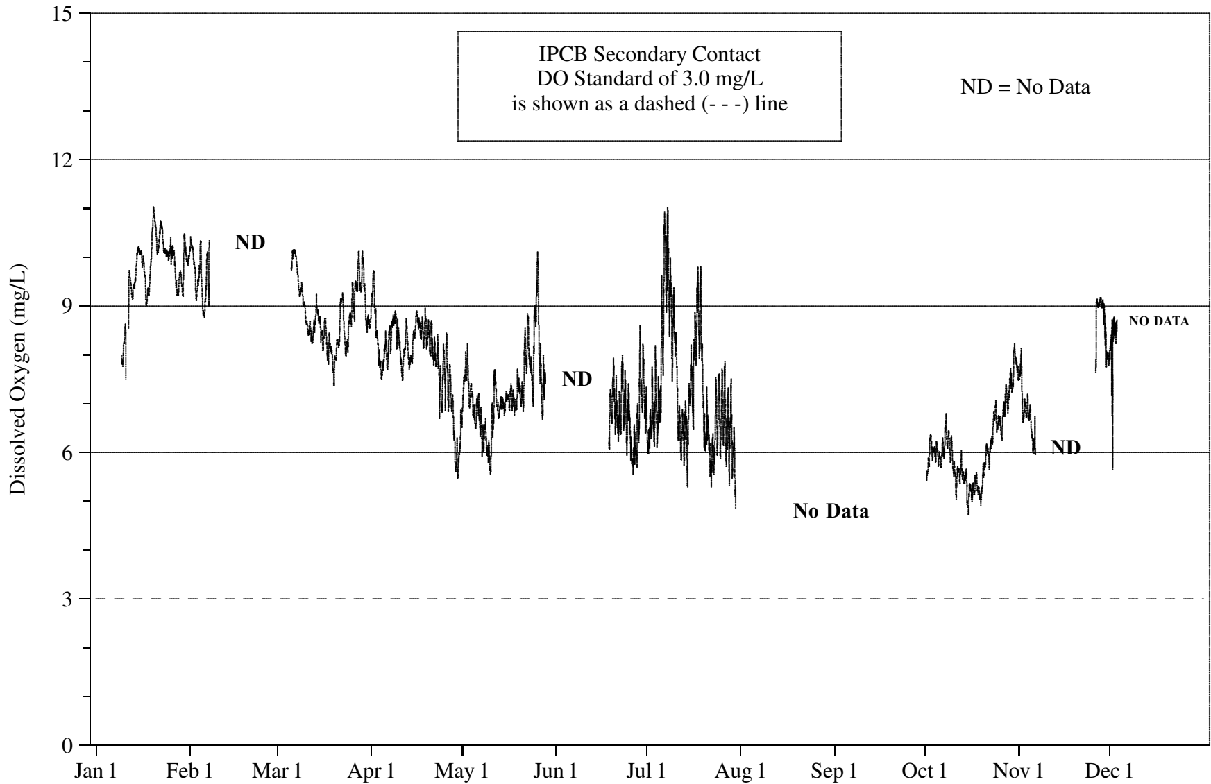
FIGURE 23: DISSOLVED OXYGEN CONCENTRATION MEASURED HOURLY AT 104TH AVENUE ON THE CALUMET-SAG CHANNEL FROM JANUARY 1, 2008 THROUGH DECEMBER 31, 2008
