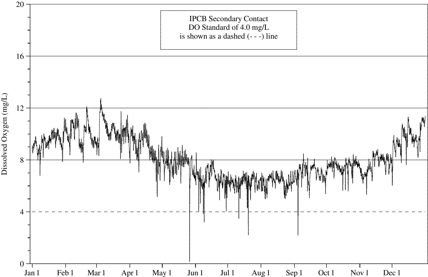
FIGURE 4: DISSOLVED OXYGEN CONCENTRATION MEASURED HOURLY AT ADDISON STREET ON THE NORTH BRANCH CHICAGO RIVER FROM JANUARY 1, 2008 THROUGH DECEMBER 31, 2008
