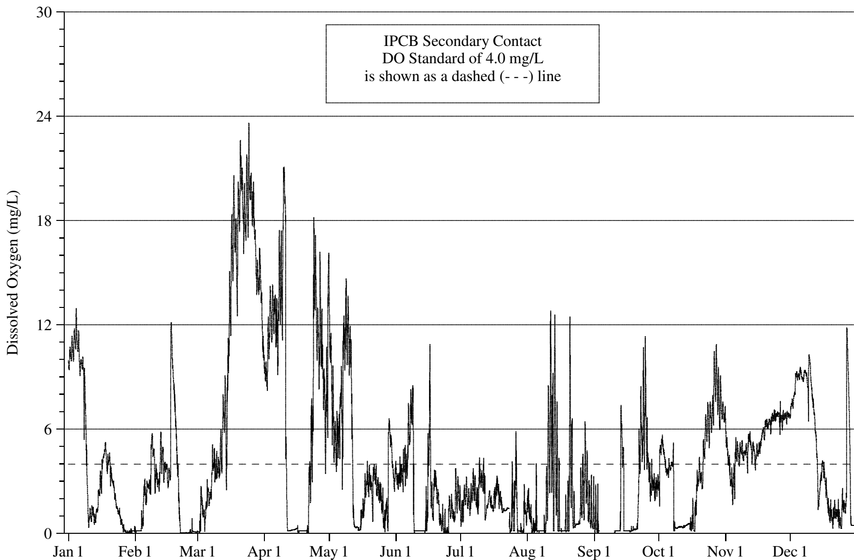
FIGURE 9: DISSOLVED OXYGEN CONCENTRATION MEASURED HOURLY AT 36TH STREET ON BUBBLY CREEK FROM JANUARY 1, 2008 THROUGH DECEMBER 31, 2008
