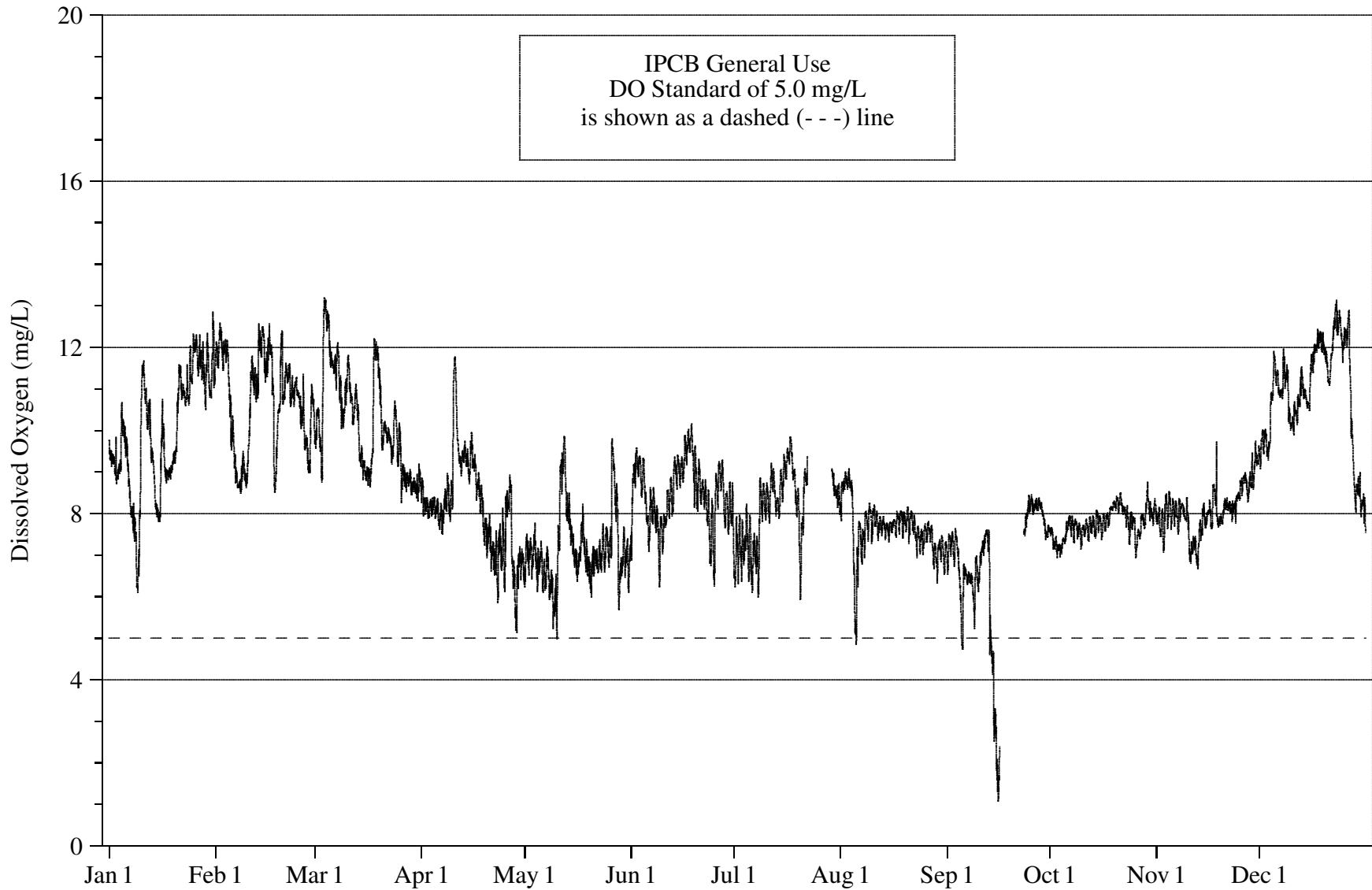
FIGURE 7: DISSOLVED OXYGEN CONCENTRATION MEASURED HOURLY AT CLARK STREET ON THE CHICAGO RIVER FROM JANUARY 1, 2008 THROUGH DECEMBER 31, 2008
