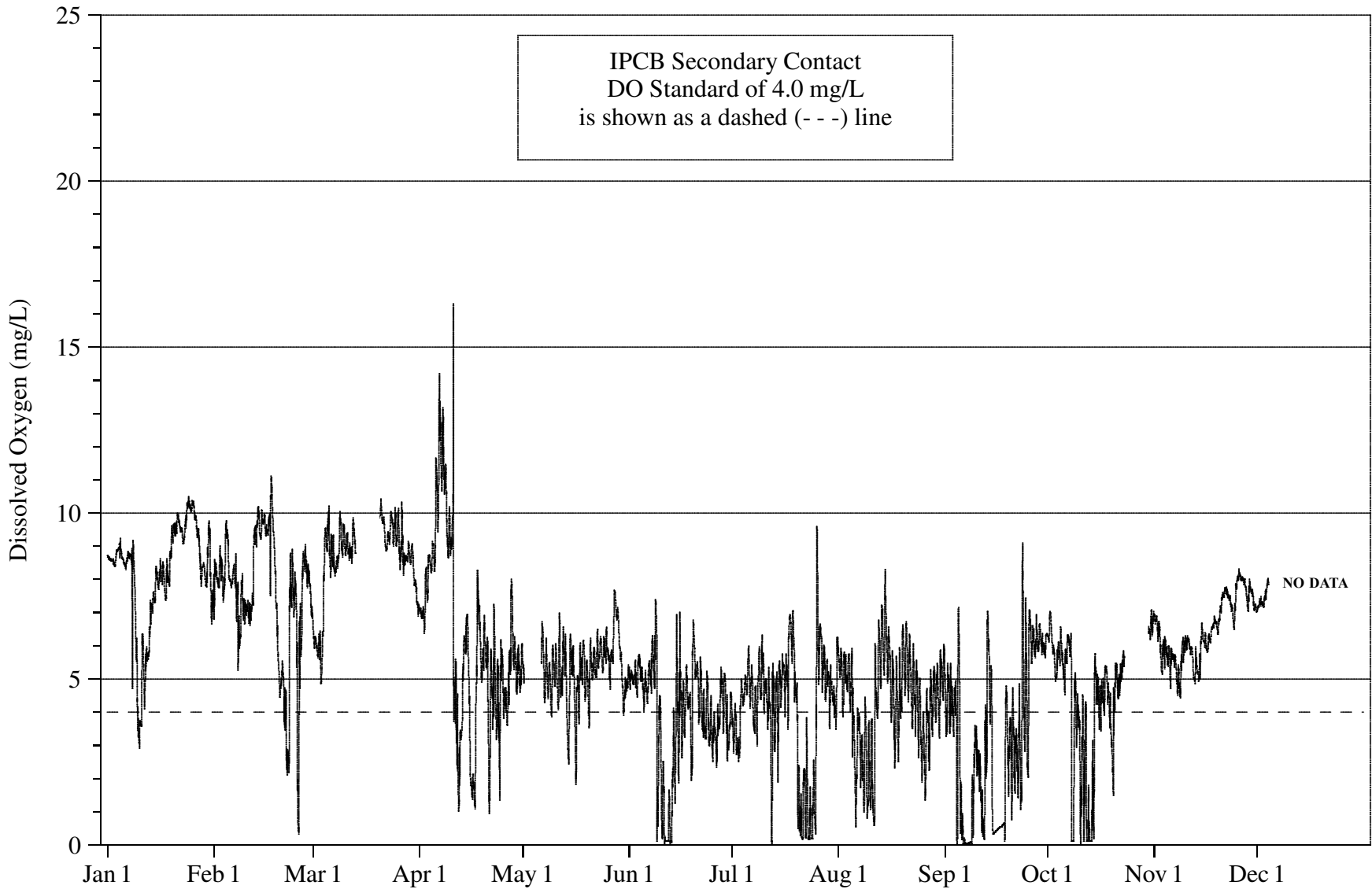
FIGURE 10: DISSOLVED OXYGEN CONCENTRATION MEASURED HOURLY AT INTERSTATE HIGHWAY 55 ON BUBBLY CREEK FROM JANUARY 1, 2008 THROUGH DECEMBER 31, 2008
