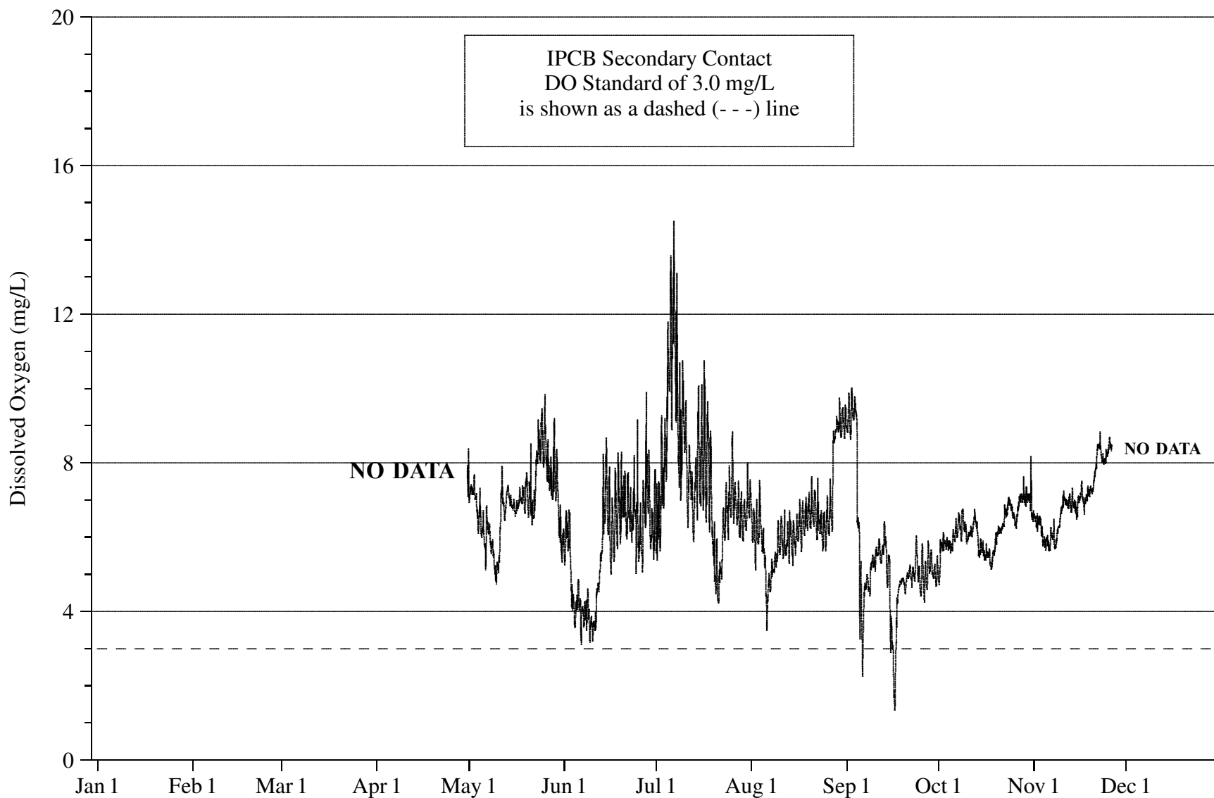
FIGURE 21: DISSOLVED OXYGEN CONCENTRATION MEASURED HOURLY AT RIVER MILE 311.7 ON THE CALUMET-SAG CHANNEL FROM JANUARY 1, 2008 THROUGH DECEMBER 31, 2008
