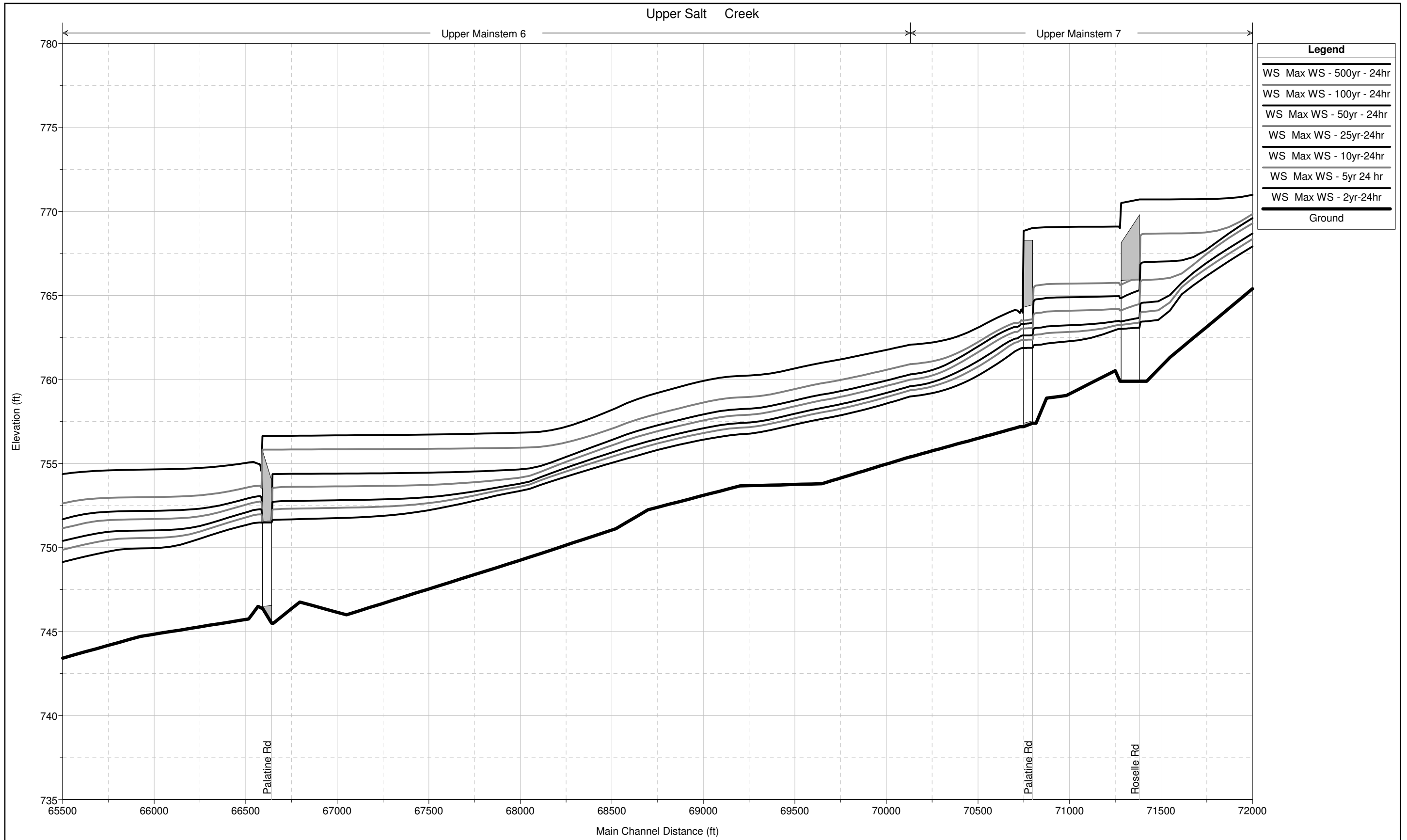
This figure is a hydrograph showing the water surface elevation (WS) in feet (ft) versus the main channel distance in feet (ft) for Upper Salt Creek. The graph is divided into two mainstem sections: Upper Mainstem 6 (from 65500 ft to 70000 ft) and Upper Mainstem 7 (from 70000 ft to 72000 ft). The y-axis represents Elevation (ft) ranging from 735 to 780. The x-axis represents Main Channel Distance (ft) ranging from 65500 to 72000. The legend indicates that the curves represent the maximum WS for various return periods: 500yr, 100yr, 50yr, 25yr, 10yr, 5yr, and 2yr, all for a 24-hour duration. The ground elevation is also shown as a thick black line. Road crossings are marked at Palatine Rd (around 66600 ft and 70800 ft) and Roselle Rd (around 71300 ft).
