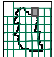
Appendix A - FIRM Panel: 17031C0044J Comparison of DWP 100-yr Inundation Mapping and FEMA Effective FIRM Upper Salt Creek Detailed Watershed Plan
