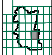
Appendix A - FIRM Panel: 17031C0192J Comparison of DWP 100-yr Inundation Mapping and FEMA Effective FIRM Upper Salt Creek Detailed Watershed Plan
