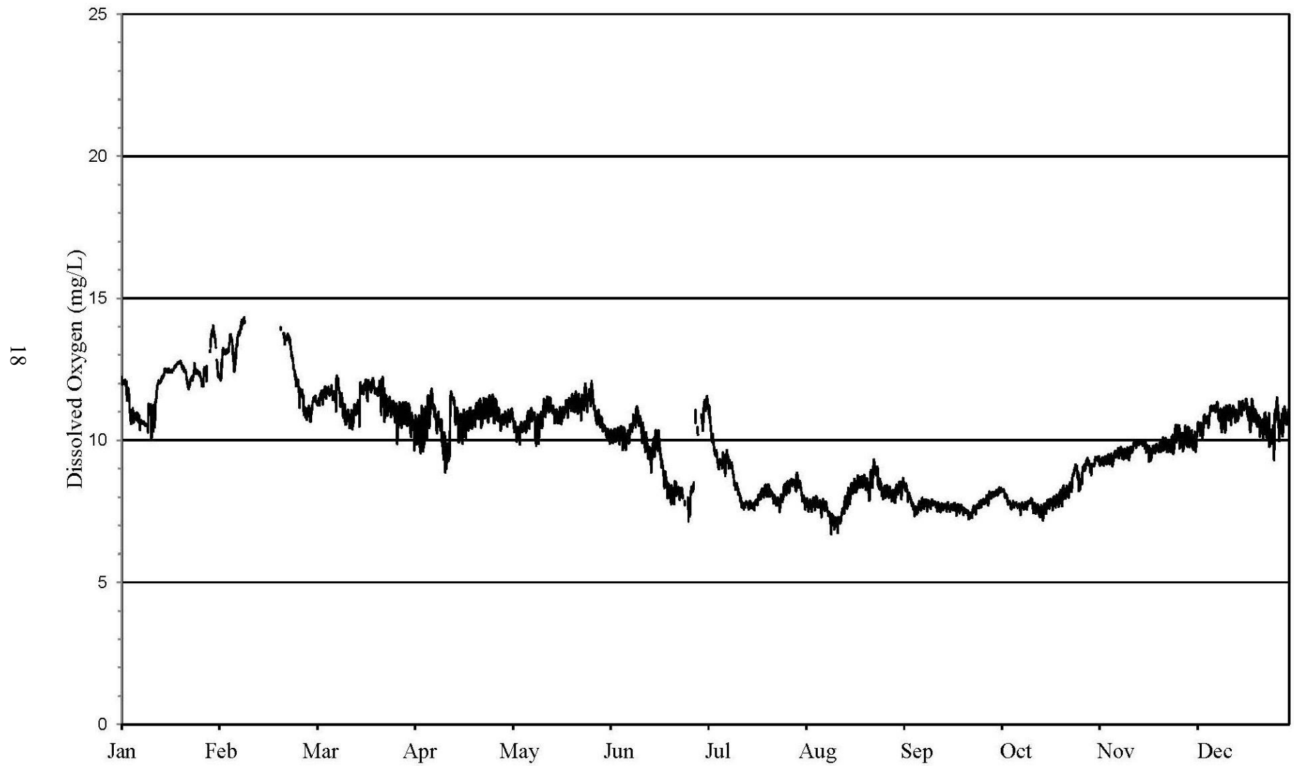
FIGURE 6: DISSOLVED OXYGEN CONCENTRATION MEASURED HOURLY AT MICHIGAN AVENUE ON THE CHICAGO RIVER FROM JANUARY 1, 2021 THROUGH DECEMBER 31, 2021
