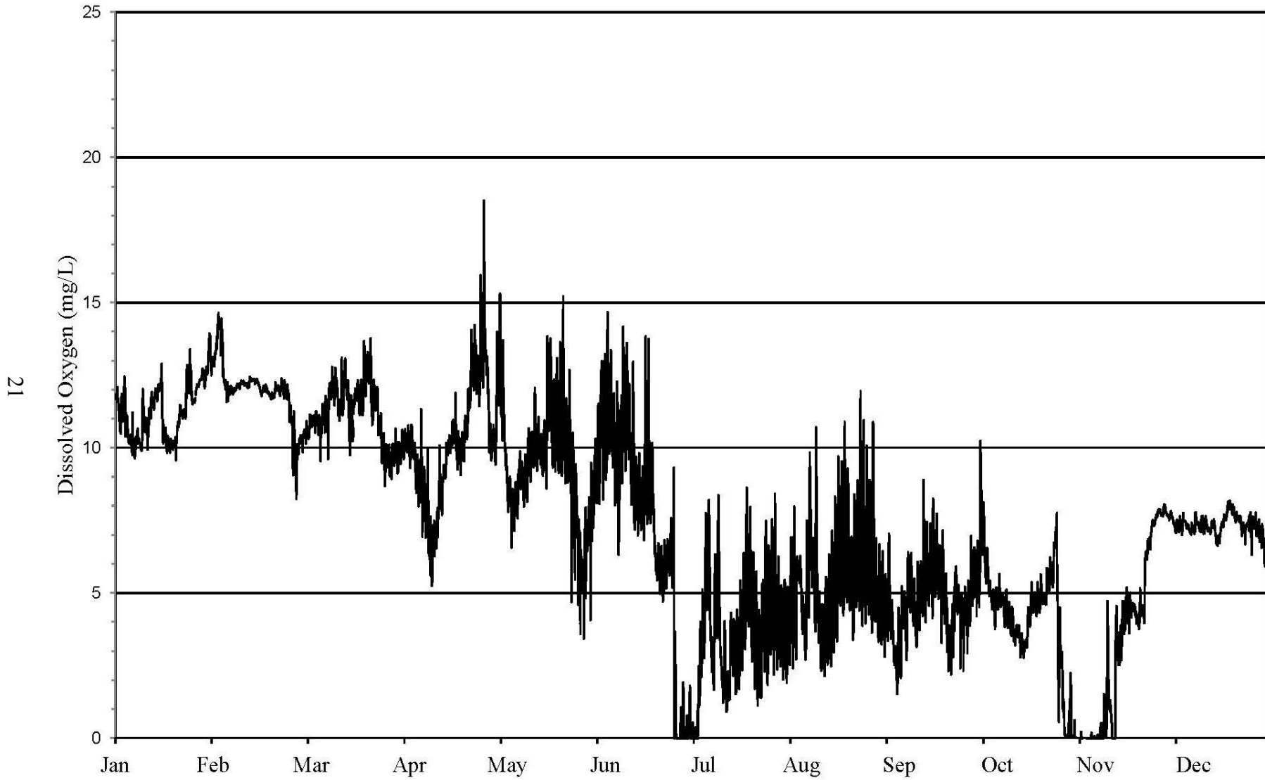
FIGURE 9: DISSOLVED OXYGEN CONCENTRATION MEASURED HOURLY AT INTERSTATE HIGHWAY 55 ON BUBBLY CREEK FROM JANUARY 1, 2021 THROUGH DECEMBER 31, 2021
