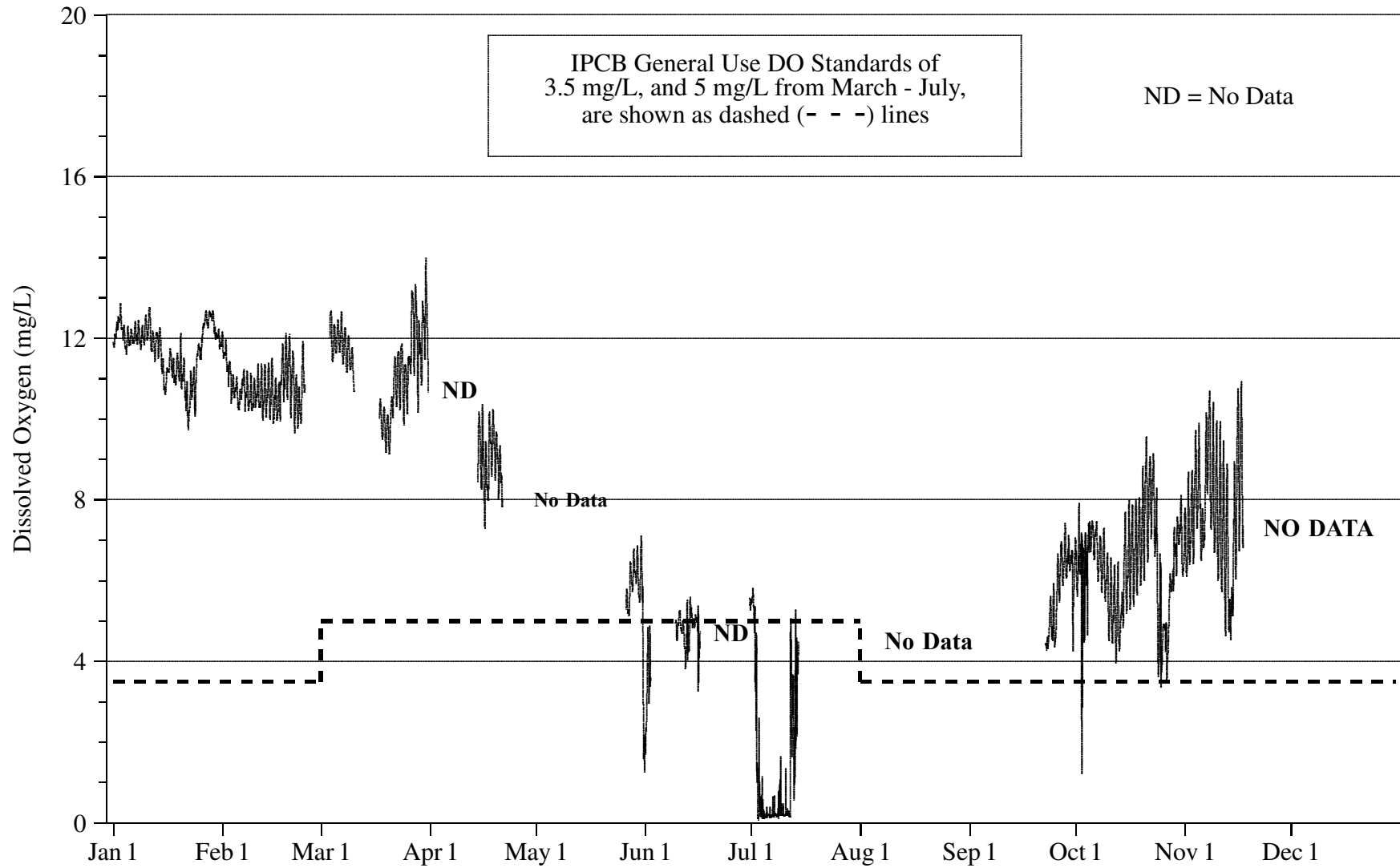
FIGURE 12: DISSOLVED OXYGEN CONCENTRATION MEASURED HOURLY AT WENTWORTH AVENUE ON THE LITTLE CALUMET RIVER FROM JANUARY 1, 2010, THROUGH DECEMBER 31, 2010
