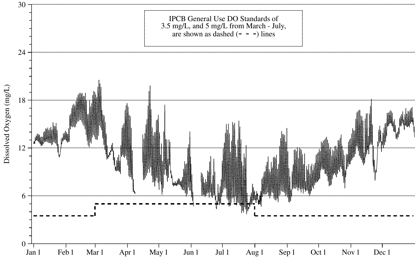
FIGURE 6: DISSOLVED OXYGEN CONCENTRATION MEASURED HOURLY AT MATERIAL SERVICE ROAD ON THE DES PLAINES RIVER FROM JANUARY 1, 2010, THROUGH DECEMBER 31, 2010
