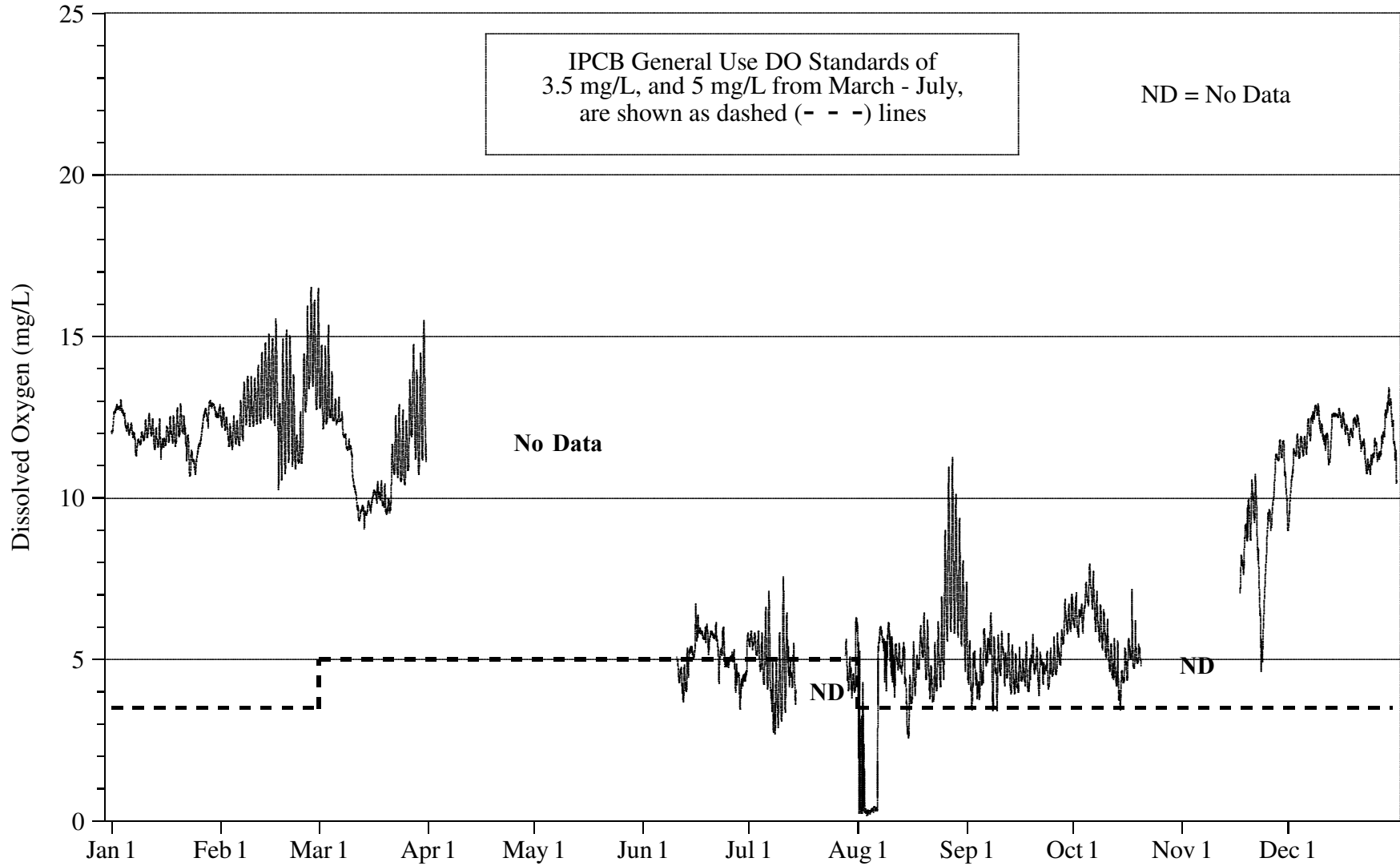
FIGURE 11: DISSOLVED OXYGEN CONCENTRATION MEASURED HOURLY AT ASHLAND AVENUE ON THE LITTLE CALUMET RIVER FROM JANUARY 1, 2010, THROUGH DECEMBER 31, 2010
