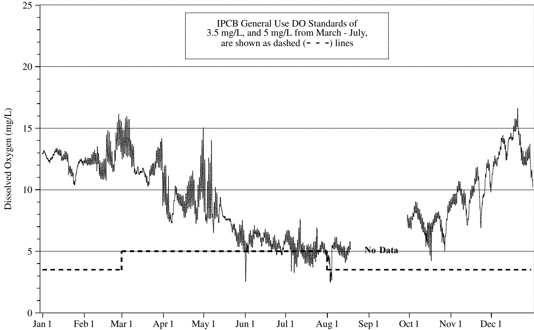
FIGURE 4: DISSOLVED OXYGEN CONCENTRATION MEASURED HOURLY AT IRVING PARK ROAD ON THE DES PLAINES RIVER FROM JANUARY 1, 2010, THROUGH DECEMBER 31, 2010
