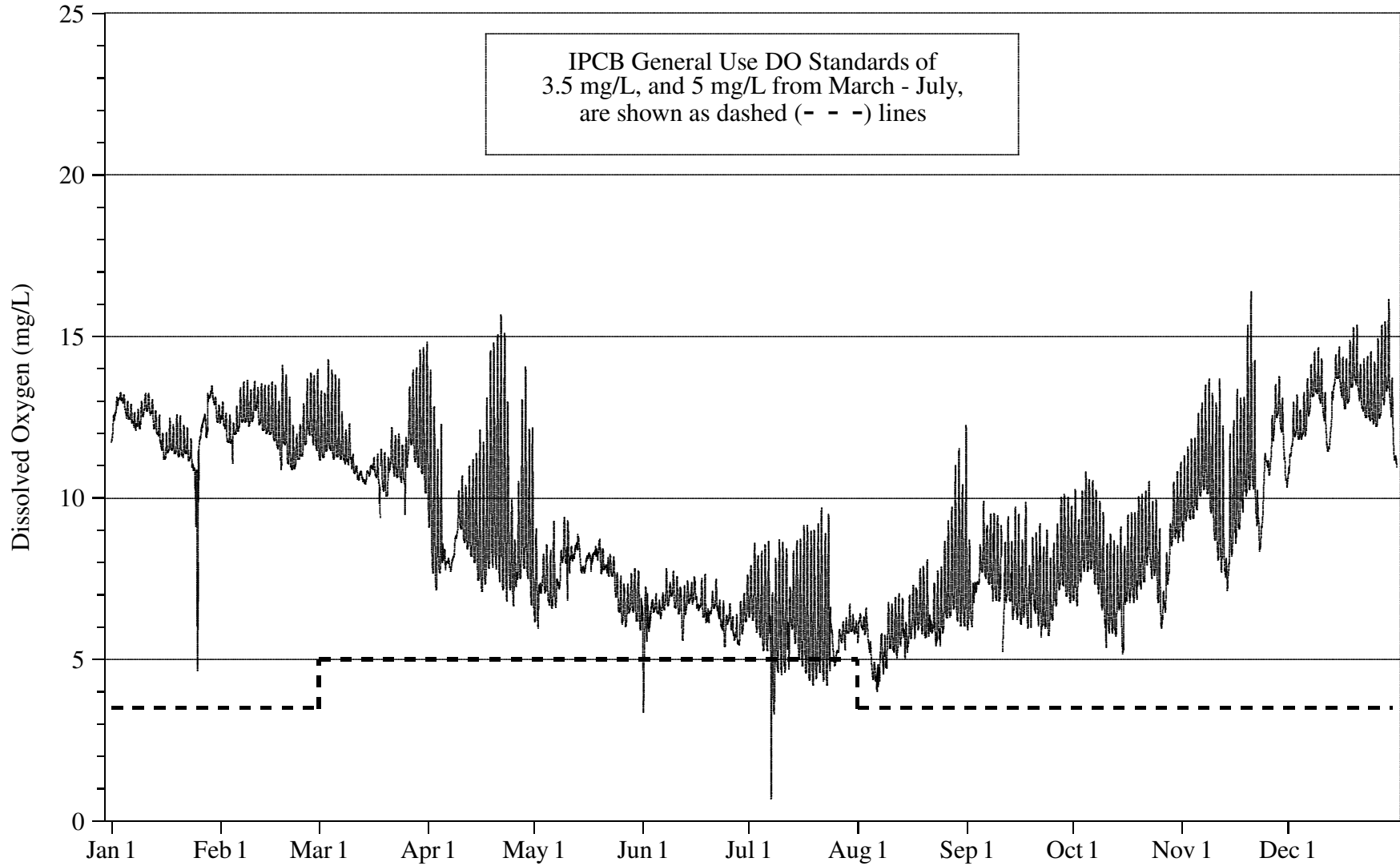
FIGURE 9: DISSOLVED OXYGEN CONCENTRATION MEASURED HOURLY AT WOLF ROAD ON SALT CREEK FROM JANUARY 1, 2010, THROUGH DECEMBER 31, 2010
