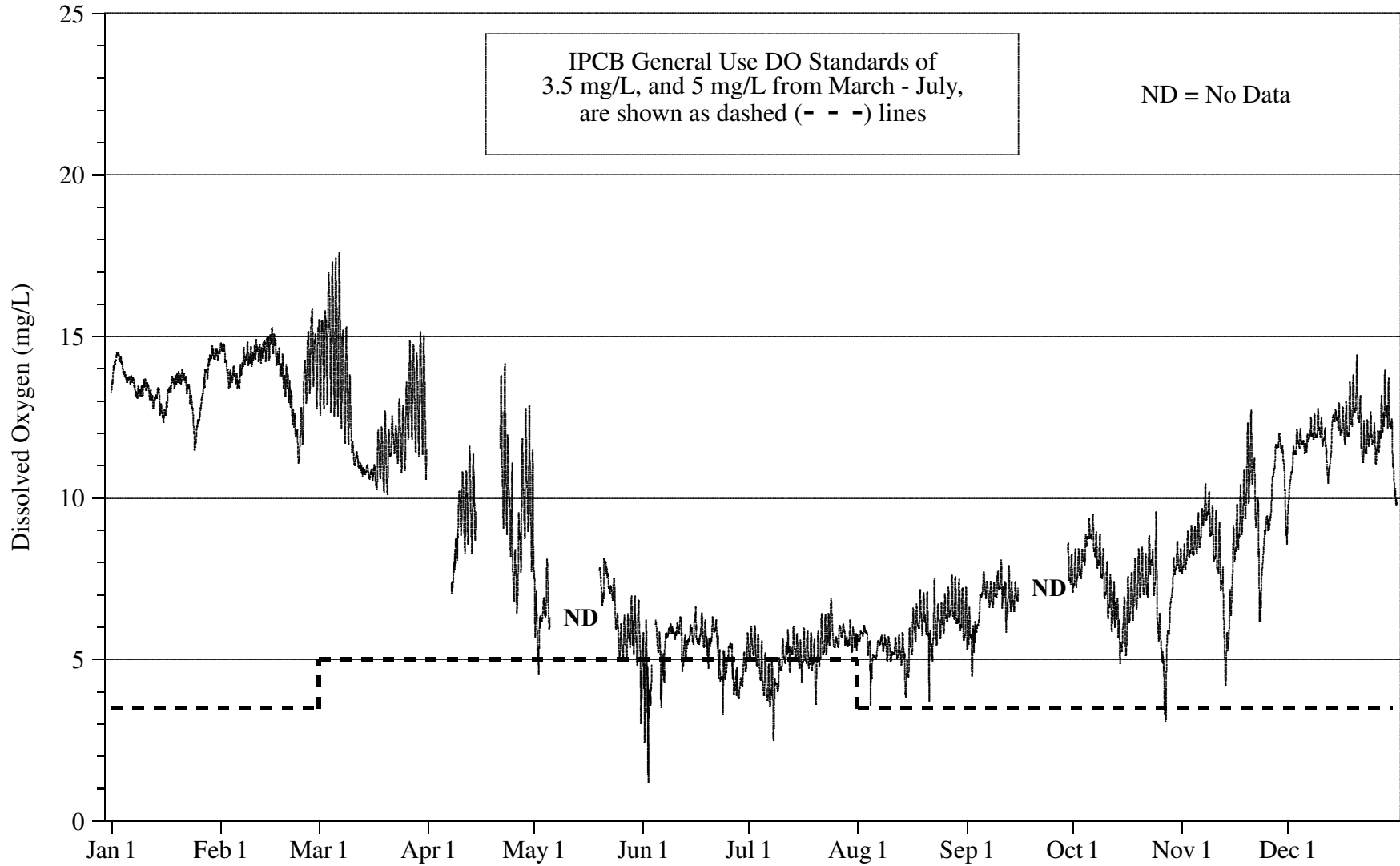
FIGURE 2: DISSOLVED OXYGEN CONCENTRATION MEASURED HOURLY AT CENTRAL PARK AVENUE ON THE NORTH BRANCH CHICAGO RIVER FROM JANUARY 1, 2010, THROUGH DECEMBER 31, 2010
