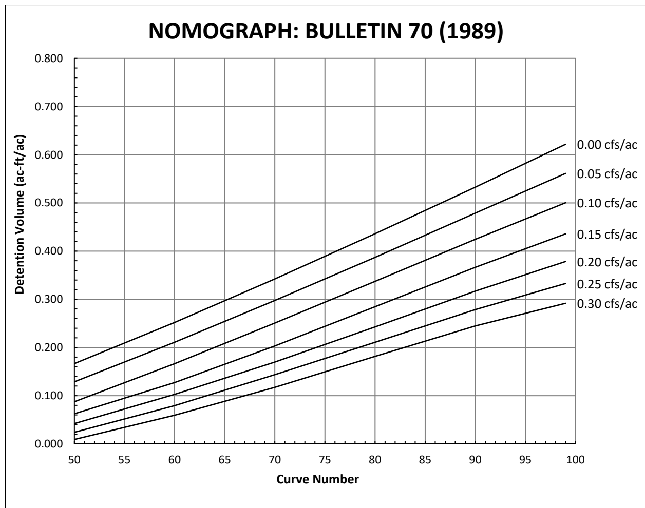
FIGURE 5.1 NOMOGRAPH FOR BULLETIN 70 (1989) RAINFALL DATA
