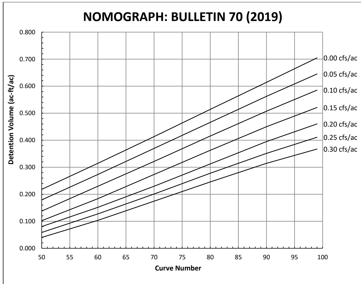
FIGURE 5.2: NOMOGRAPH FOR BULLETIN 70 (2019) RAINFALL DATA
