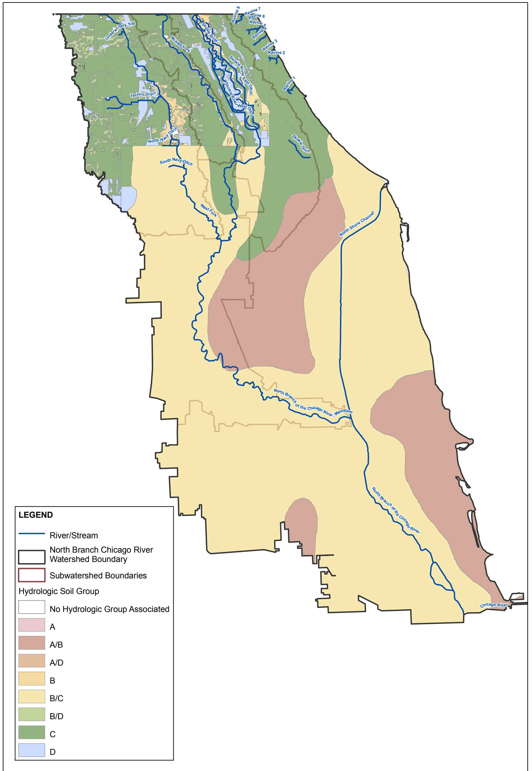
Figure 2.3.4 North Branch of the Chicago River Watershed Hydrologic Soil Groups
