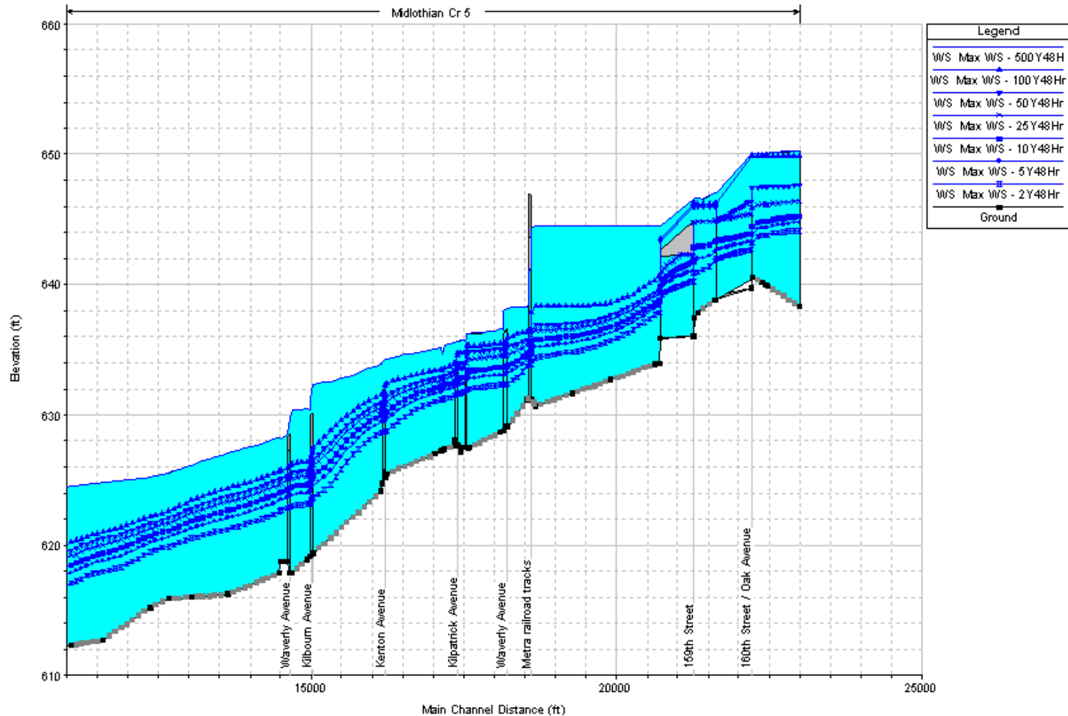
Midlothian Creek, Reach 5 (encompassing Reach 2,3 & 4) Midlothian Cr. Western Branch (at Grove Ave. & 161 st St.) to upstream of Pulaski Road
