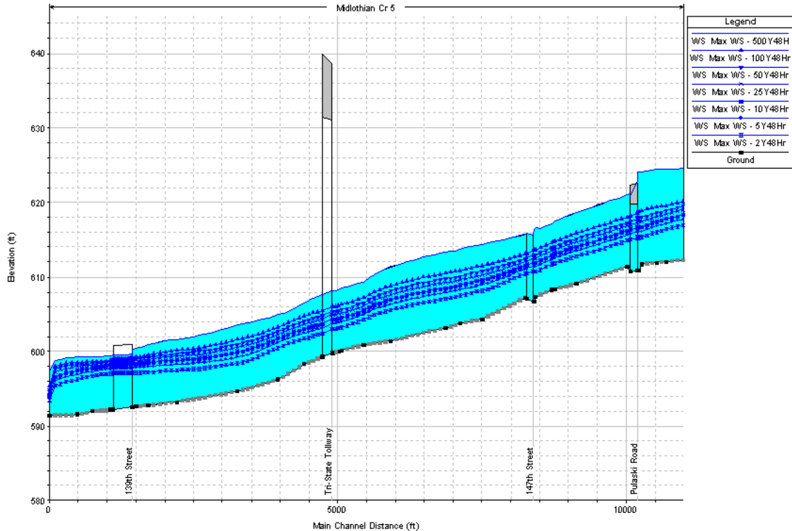
Midlothian Creek, Reach 5 (encompassing Reaches 2,3,& 4) Pulaski Road to confluence with Midlothian Cr. Diversion Channel
